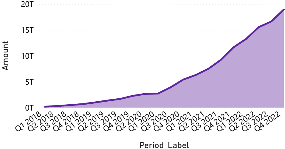
Transaction Amount Trend (2018-2022)
